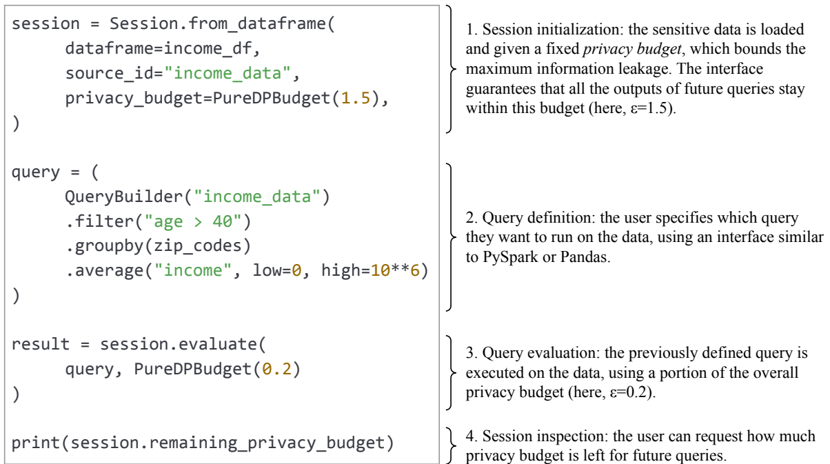
Figure 1: An annotated Tumult Analytics program that computes the average income of all people older than 40 in an input dataframe income_df , grouped by ZIP code.
