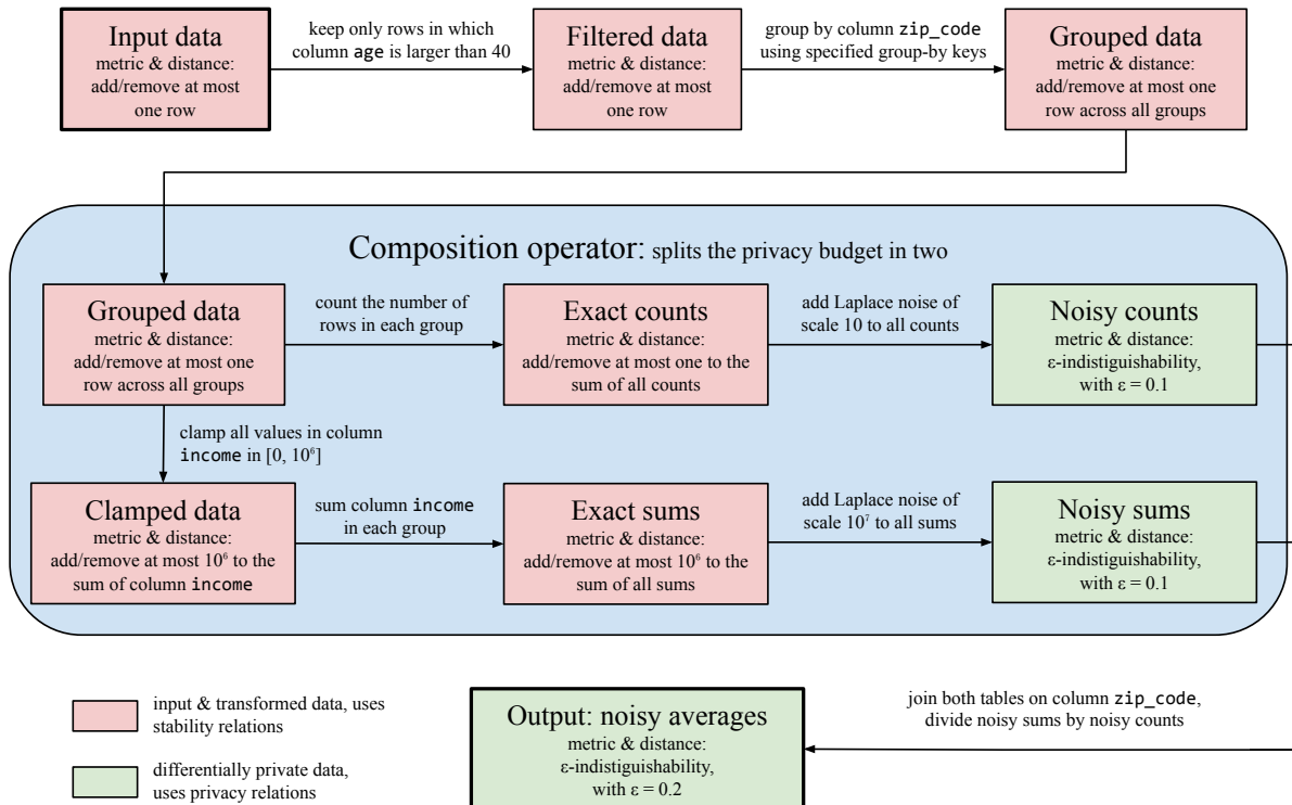
Figure 2: A simplified diagram outlining the steps taken by the data through Tumult Core transformations, measurements and operators, to implement the query in Figure 1. Each labeled arrow corresponds to a Core component. The actual series of Core components to implement this query is more complex and incorporates some additional optimizations.
